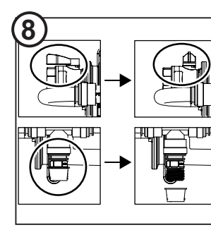
Close INLET valve and open outlet valve.
