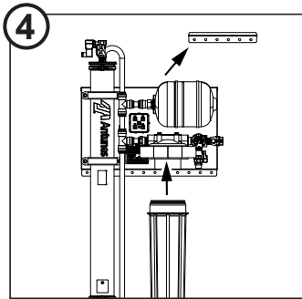
4 Hang system and install empty carbon bowl.
