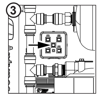
3 Push FLUSH button 6 times.
