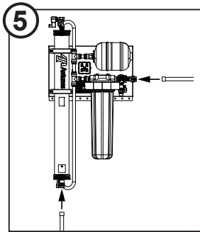
5 Connect inlet and outlet plumbing.
