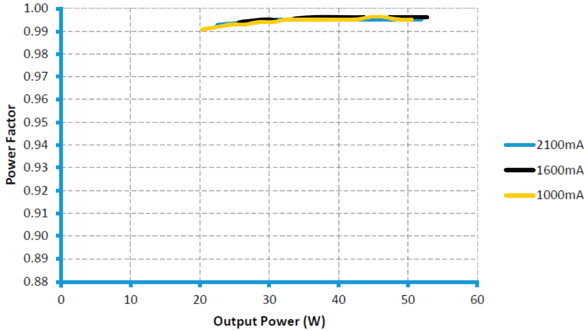
Power Factor vs Output Power (120V)
