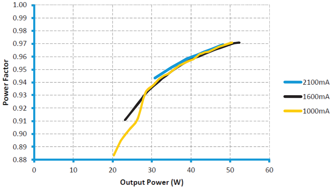
Power Factor vs Output Power (277V)
