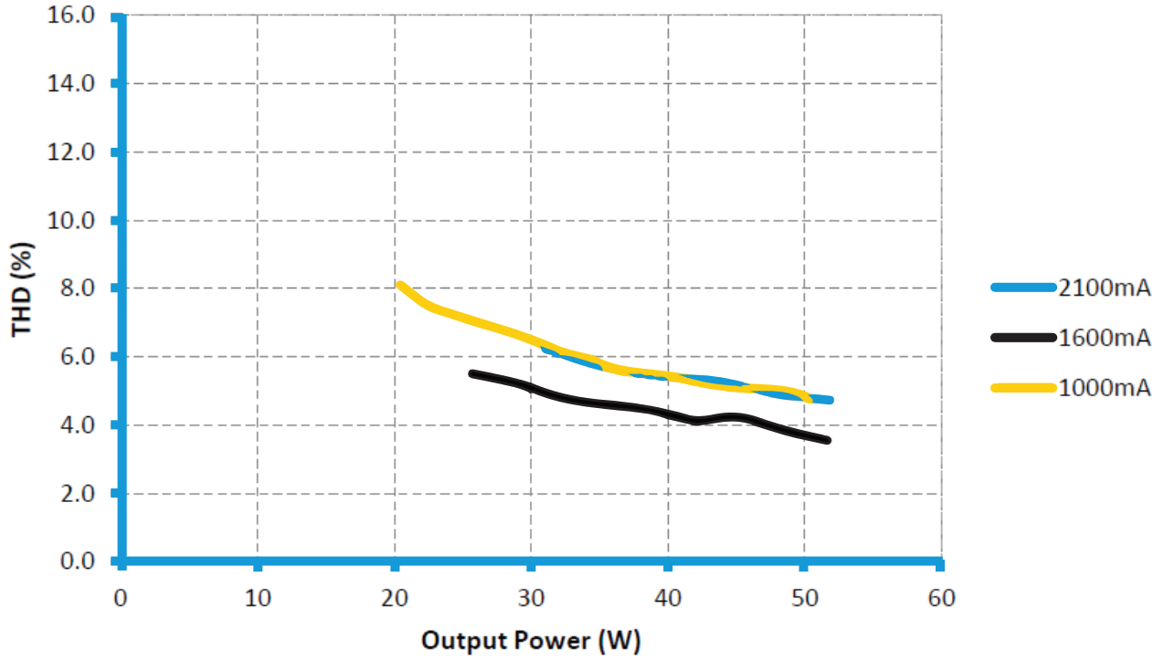
THD vs Output Power (277V)
