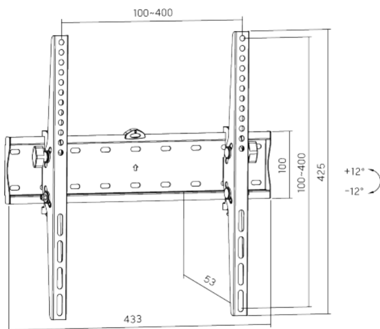
Dimensions (mm)
