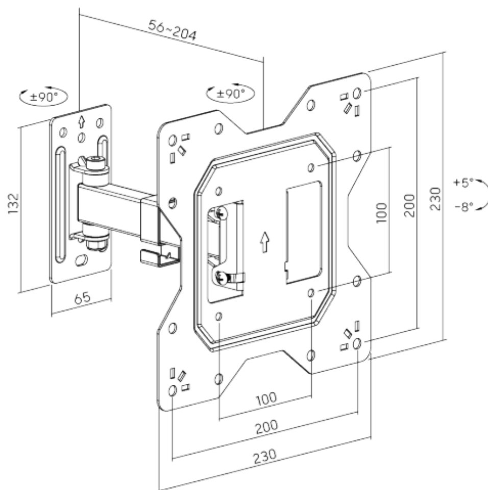
Dimensions (mm)
