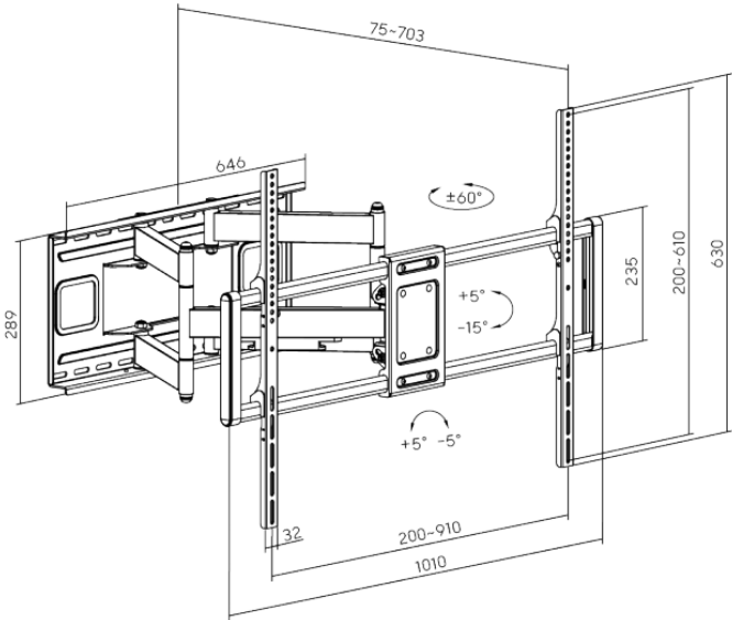
Dimensions (mm)
