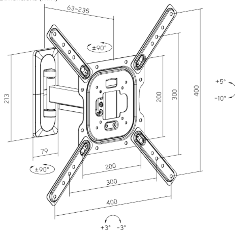
Dimensions (mm)
