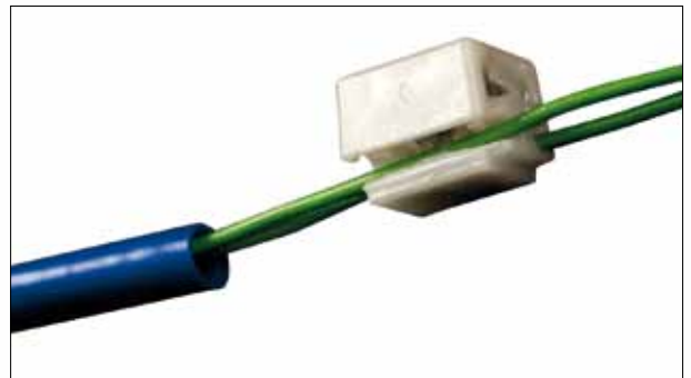
Pre-crimping to retain the 11A on the wires.
