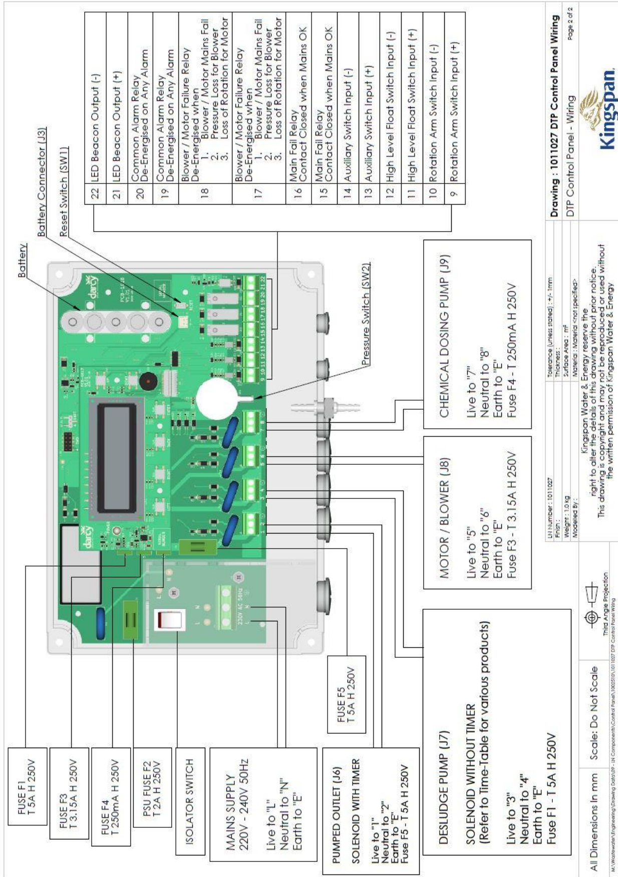
Figure 2 Wiring Diagram
