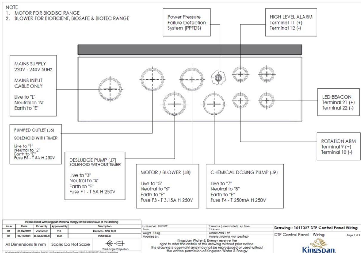
Figure 1 : Control Panel Gland Holes
