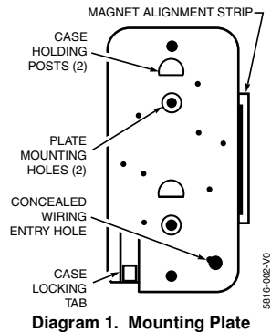
Diagram 1. Mounting Plate
