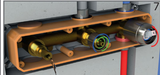
7 DAR EL AGUA Y COMPROBAR QUE NO TENGA FUGAS ANTES DE CERRAR. TURN ON THE WATER AND CHECK FOR LEAKS BEFORE SHUTTING OFF THE WATER.
