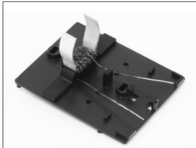
Field Coil Mounted on Base
