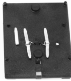
Field Coil and Brushes Wired, Underside View
