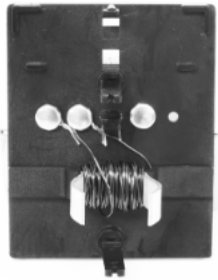
Field Coil and Brushes Wired
