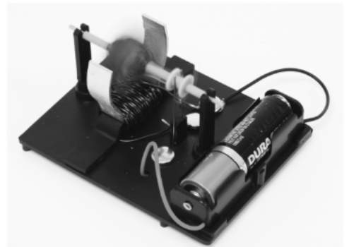
Completed Motor with Battery, in Operation
