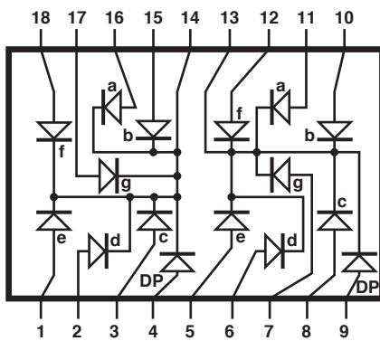
COMMON CATHODE 08TIE525
