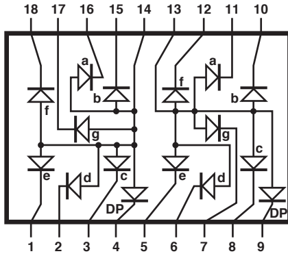
COMMON ANODE 08TIE524
