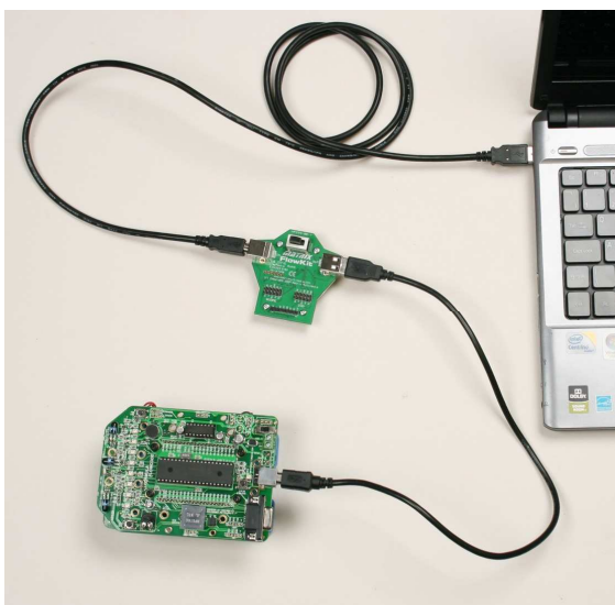
Using Flowkit with Formula Flowcode
