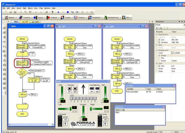
The system is controlled within Flowcode 4.2+ where the icon just executed is clearly marked
