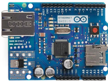
Arduino Ethernet Shield
