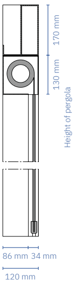
Section view A-A
