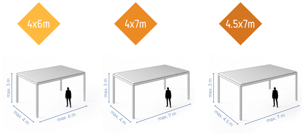
Bioclimatic Pergola SL 160/28
