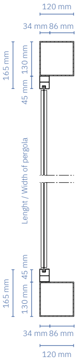
Section view B-B
