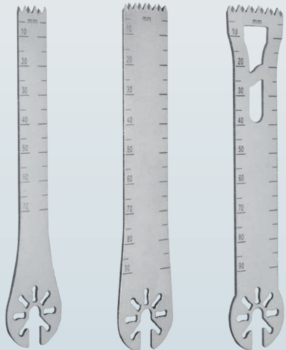
Blade, 10014015, 12.5×70×1mm Blade, 10014011, 19.5×90×1mm Blade, 10014013, 25.0×90×1mm
