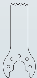
Coarse, 10017013, 9.5×25.5mm
