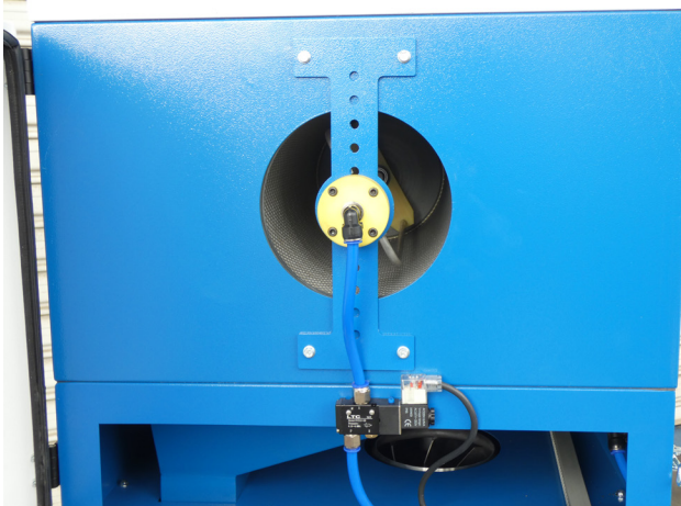
Effective Auto rotary filter cleaner
