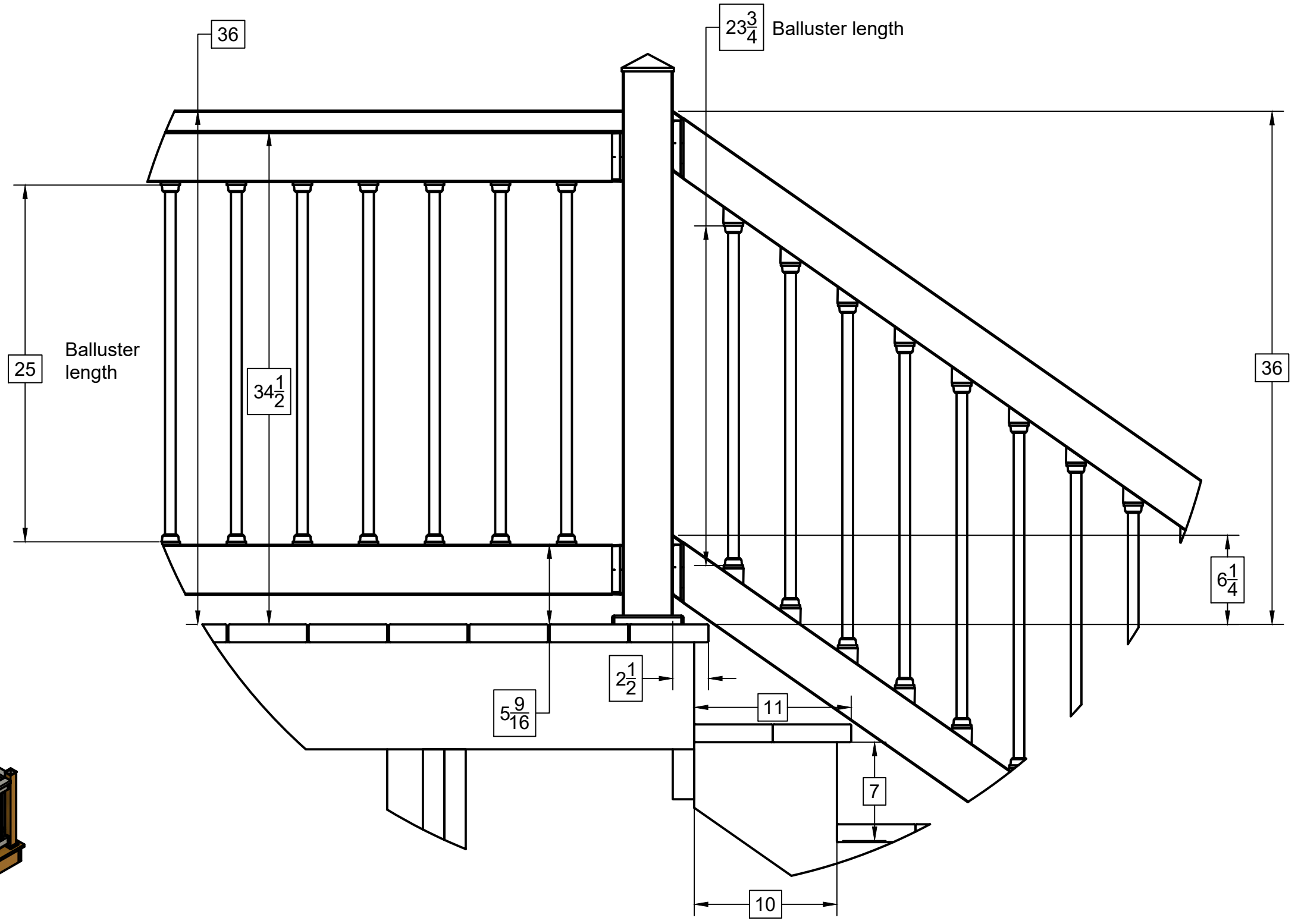
DETAIL A SCALE 1-1/2" = 1'-0"
