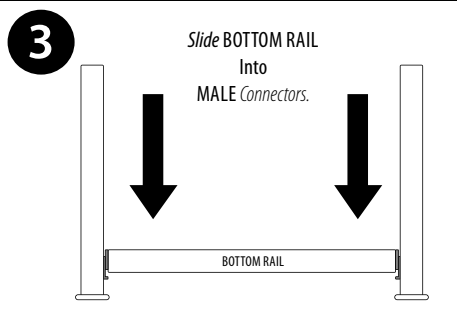
SHADOW RAIL CONNECTOR™ LEVEL ASSEMBLY
