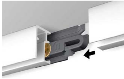
Easy to join rails together
