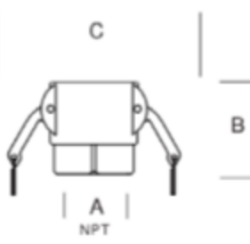
Coupler 'DC'
