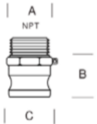
Adapter 'DP'
