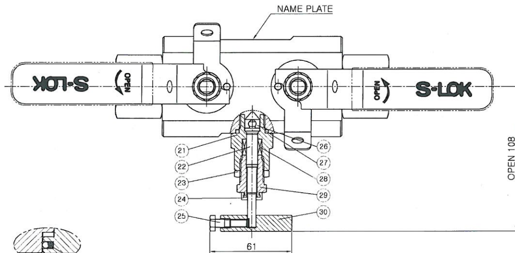
ANTI-STATIC DEVICE
