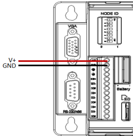
Figure 3.1 Power Supply Wiring
