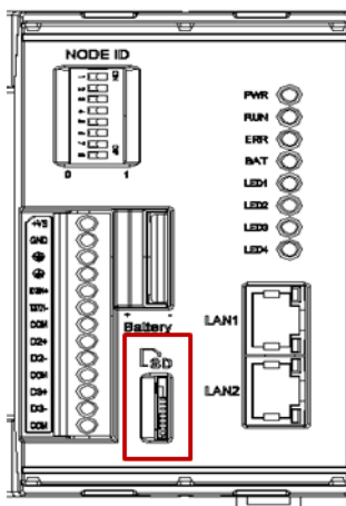
Figure 3.7 Battery replacement
