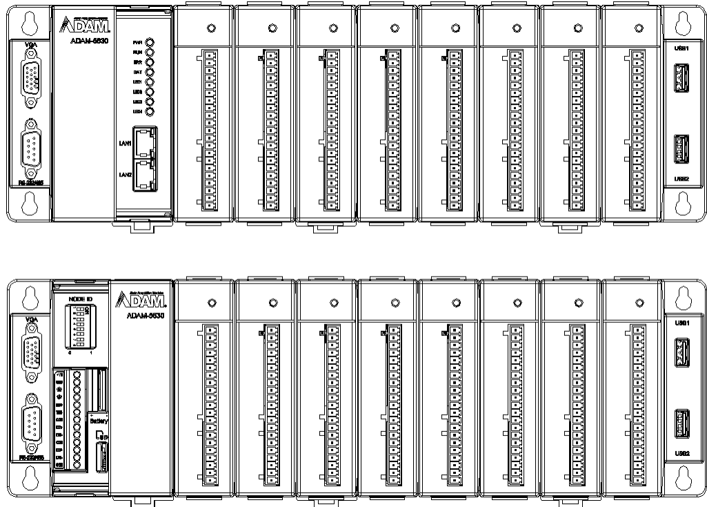
Figure 2.1 ADAM-5630E overview (the I/O module are optional, not included)
