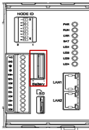
Figure 3.6 SD Card Installation
