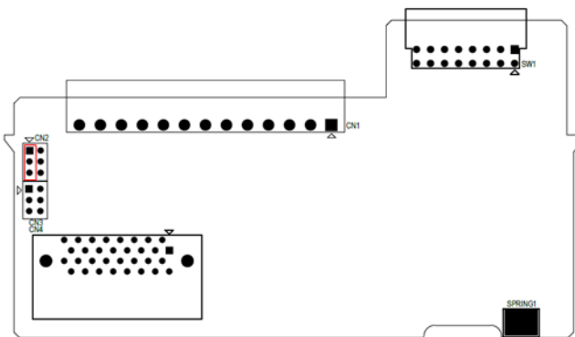
Figure 3.2 The location of Jumper on the power board
