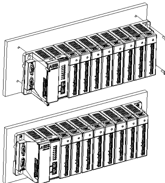
Figure 3.5 Wall mounted Installation (8 slots as example)
