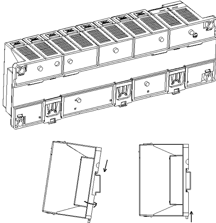
Figure 3.4 DIN-rail mounted Installation (8 slots as example)
