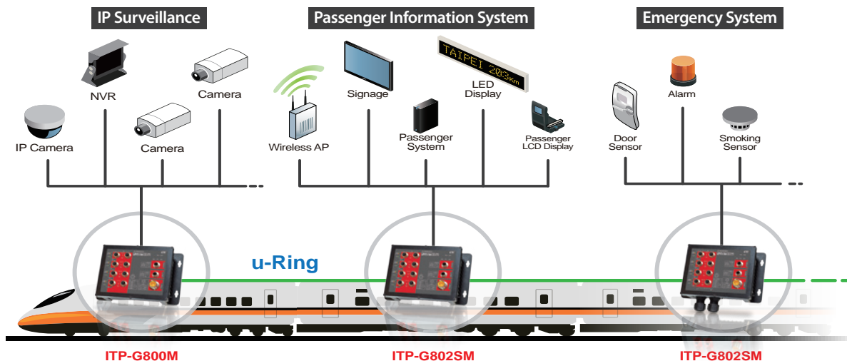
Figure 1 : ITP Series in Onboard Train Application
