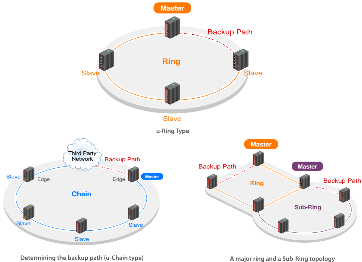
Figure 5 : u-Ring Type
