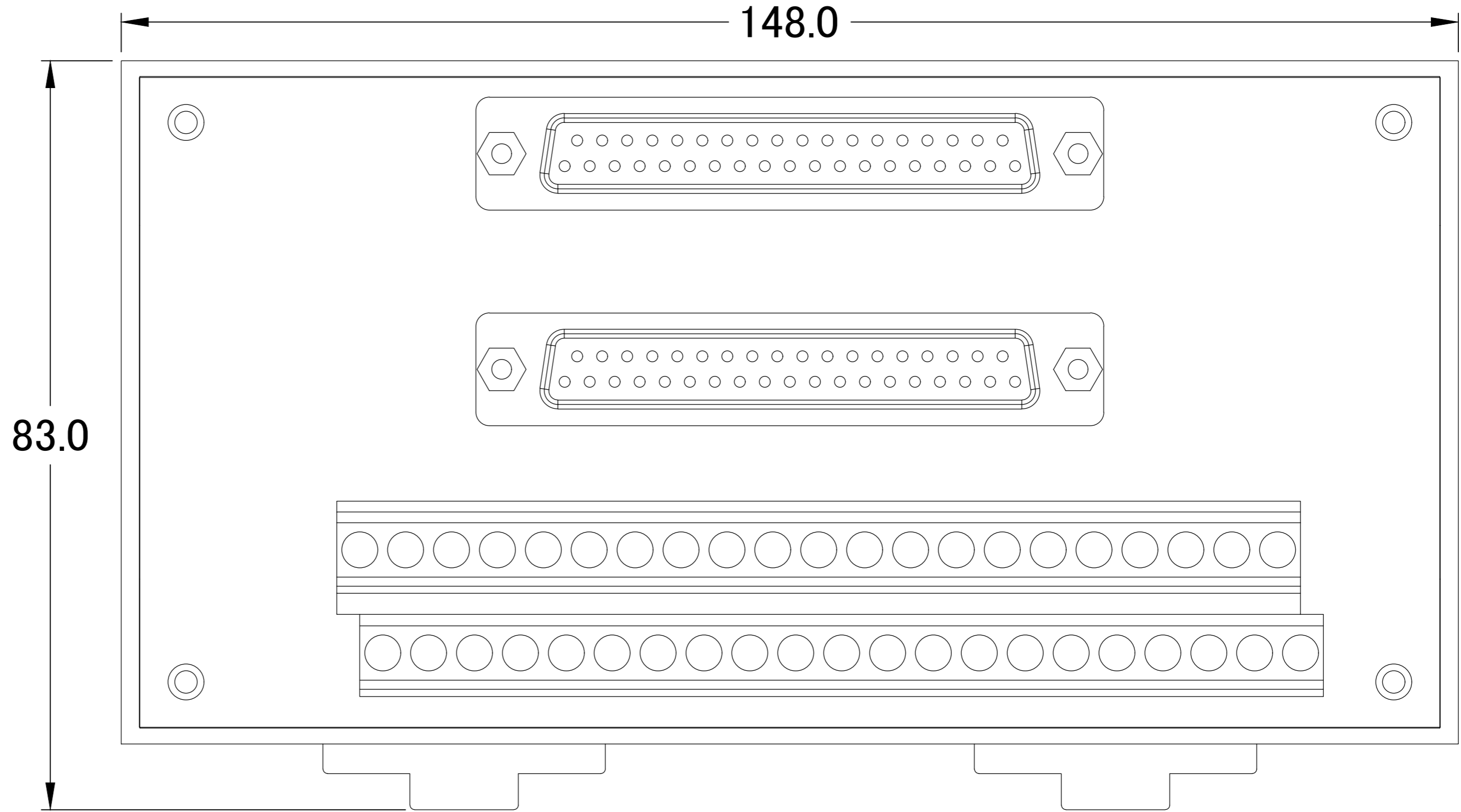
Front View
