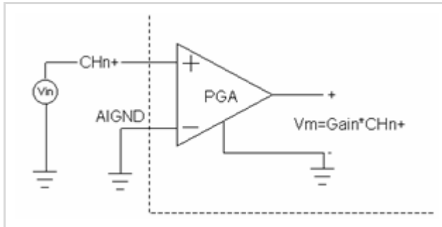
Figure 3-1: Single-Ended Connections
