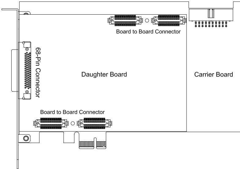
Figure 2-1: DAQe-2016/2010/2006/2005 Card Layout
