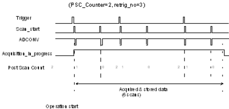
Figure 4-12: Post trigger with re-trigger
