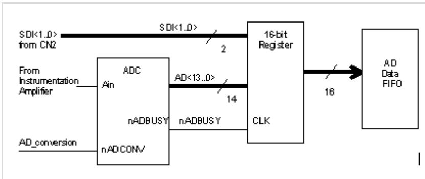
Figure 4-1: Synchronous Digital Inputs Block Diagram
