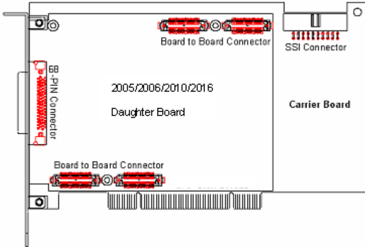
Figure 2-2: DAQ-2016/2010/2006/2005 Card Layout
