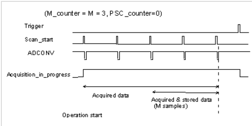
Figure 4-4: Pre-trigger
