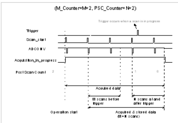
Figure 4-9: Middle-Trigger
