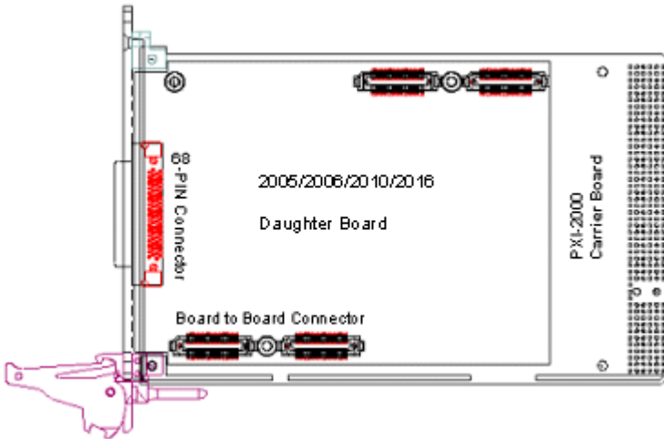
Figure 2-3: PXI-2016/2010/2006/2005 Card Layout
