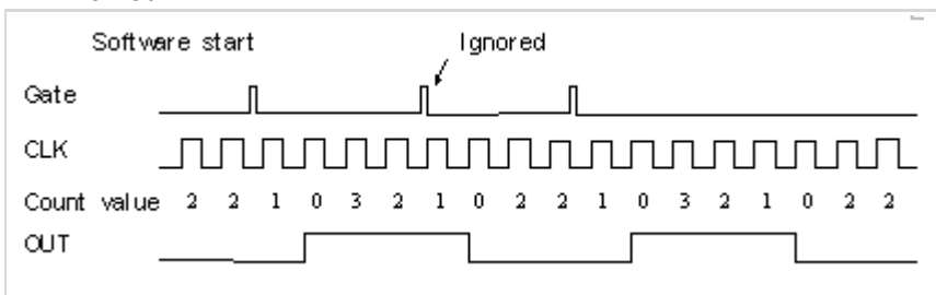
Figure 4-28: Mode 6 Operation
