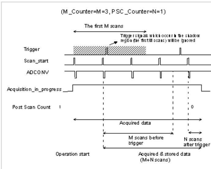
Figure 4-8: Middle-Trigger with M_enable = 1
