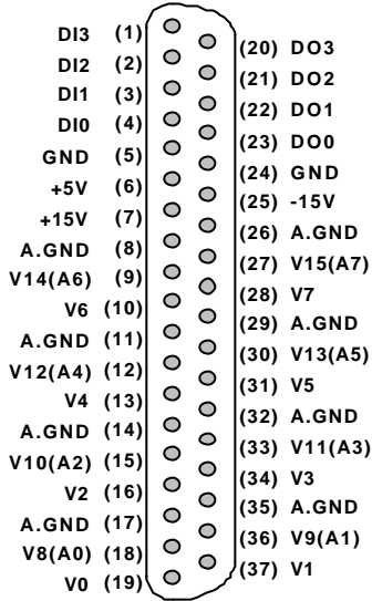
Figure 2.2 Pin Assignment of CN1 connector
