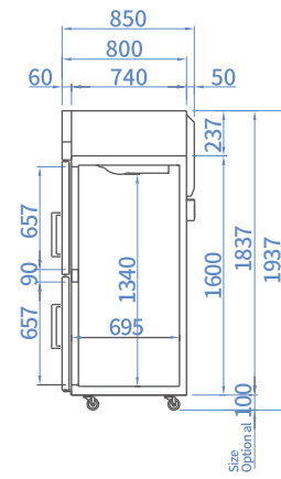
SIDE VIEW (Half glass Door)
