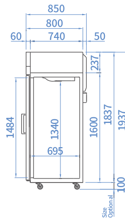
SIDE VIEW (Glass Door)
