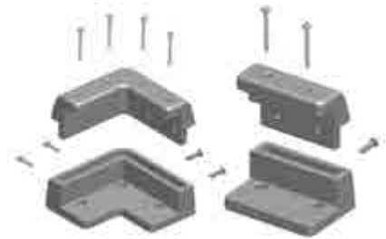
CAMEC SOLAR PANEL MOUNTING KIT 4 CORNER AND 2 SIDE BRACKETS 040436
