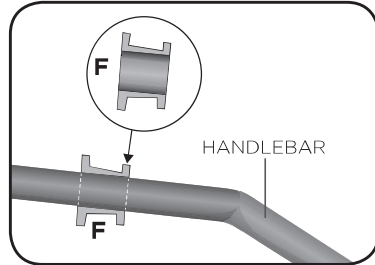
Corret position of the parts "F" on handlebar 28 mm, 1.102 inch.
