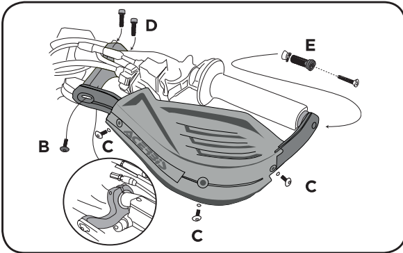
For handlebars fatbar 28 mm. / 1.102 inch.
