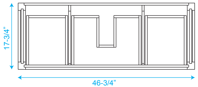
TOP VIEW OF VANITY CABINET
