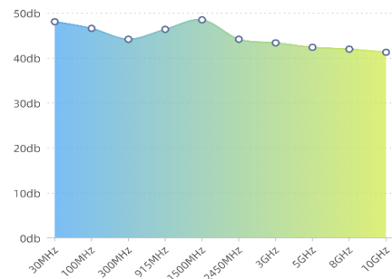
Shielding Effectiveness
