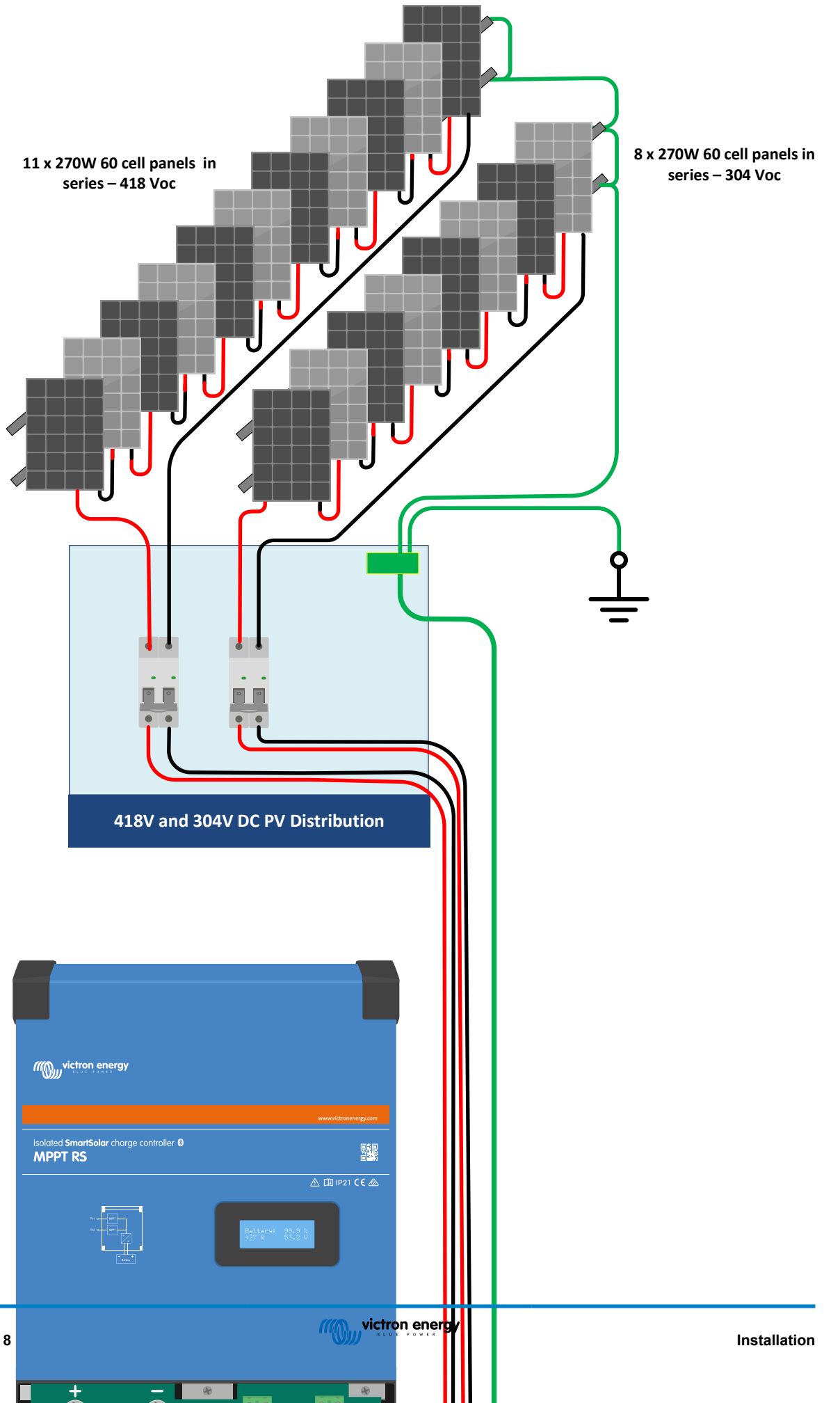
Figure 2. MPPT RS PV example diagram
