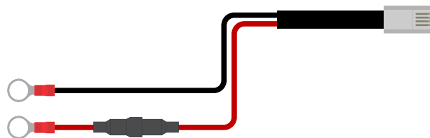
Power cable
