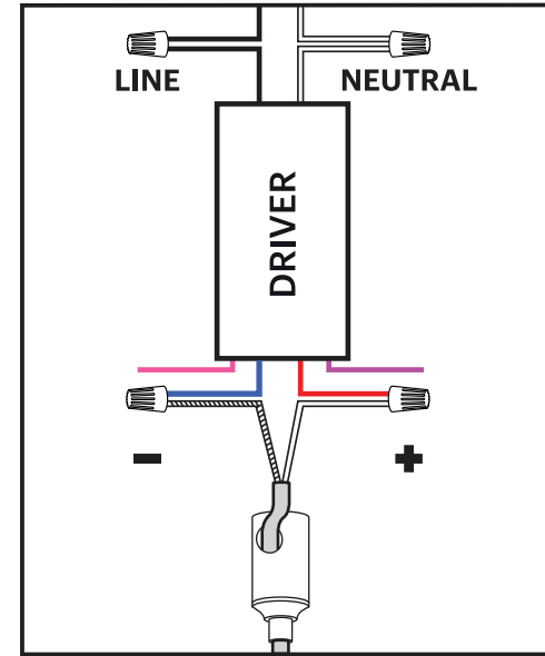
WIRING DIAGRAM
