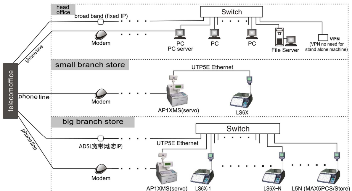
The connection diagram of Broad Band POS Cash Register (Pinnacle exclusive)
