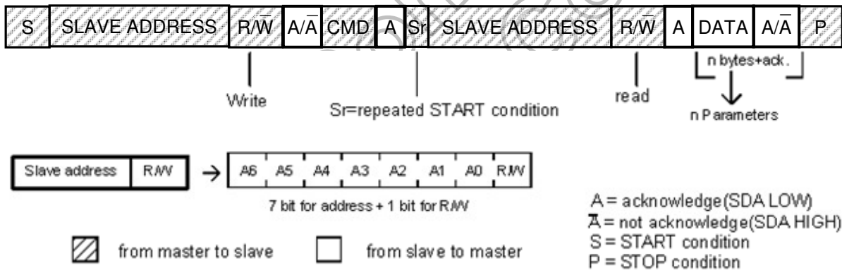
Figure 11.5: Data format of reading mode
