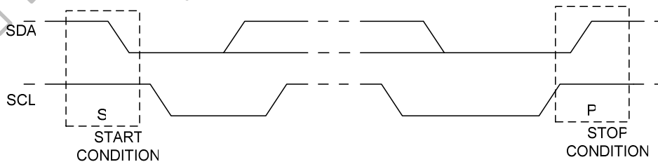
Figure 11.2: I 2 C START/STOP
