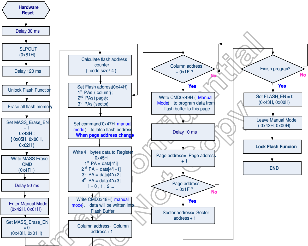
Figure 12.1: Flash programming flow
