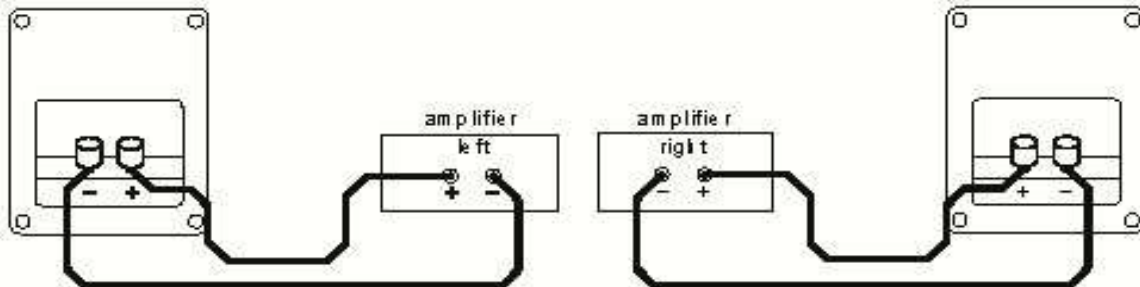
fig. 5 amplifier & terminal
