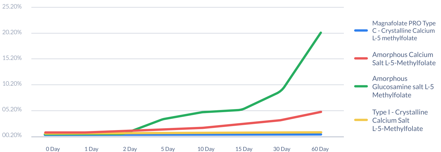
The 60-day trend chart of the impurity, 4a-Hydroxy-5-methyltetrahydrofolic acid, for the 4 compared L-Methylfolates
