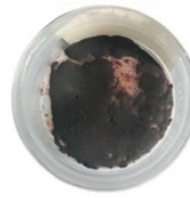
Amorphous Glucosamine Salt L-5-Methylfolate
