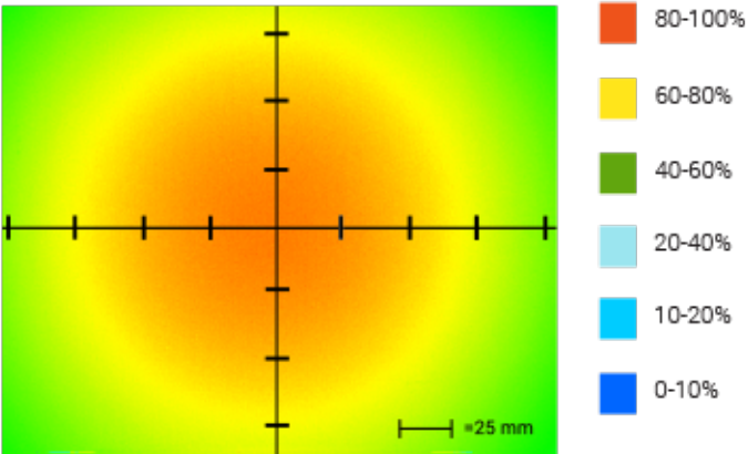
Optical measurement taken using FD0808-WHIC @ 200mm
