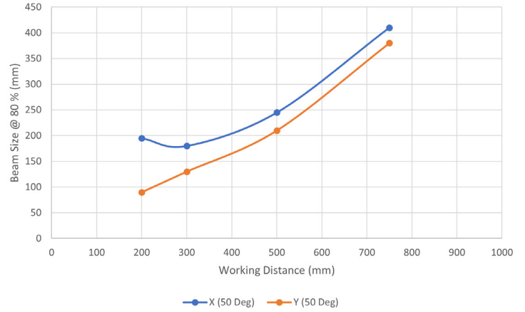
50 Deg Beam Size at 80% Max Intensity vs. Working Distance
