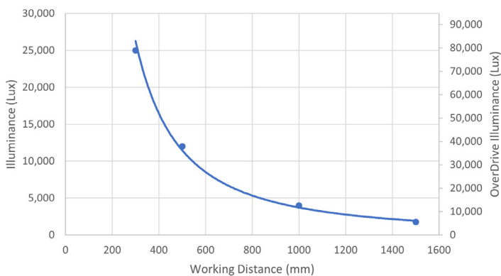
Illuminance vs. Working Distance 30 Deg
