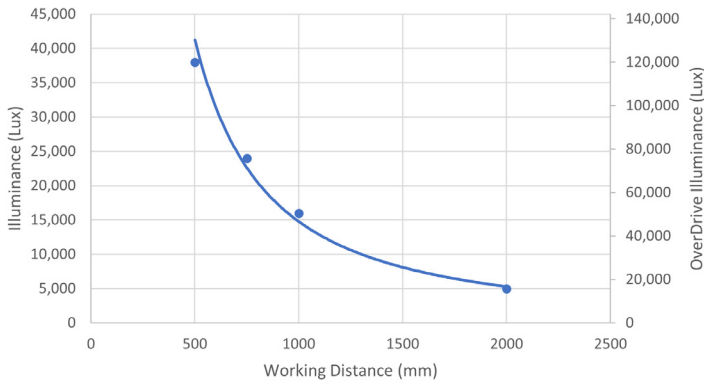
Illuminance vs. Working Distance 10 Deg
