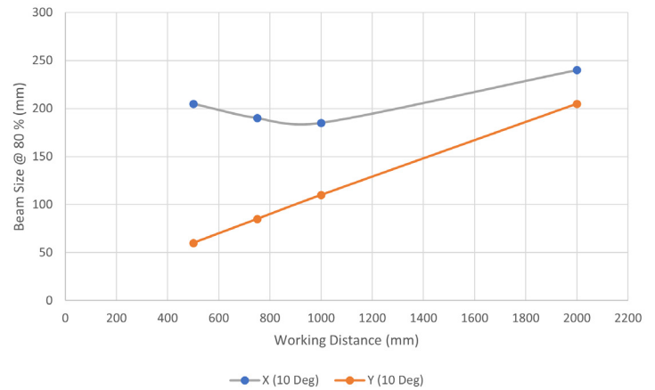
10 Deg Beam Size at 80% Max Intensity vs. Working Distance
