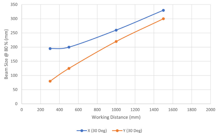
30 Deg Beam Size at 80% Max Intensity vs. Working Distance
