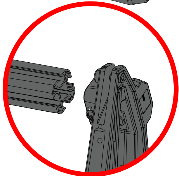
DETAIL-1
