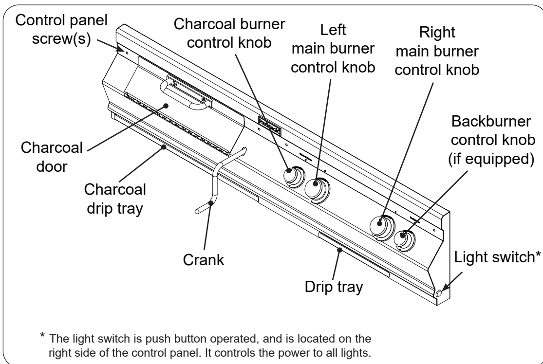
Fig. 32-1 A830 controls
