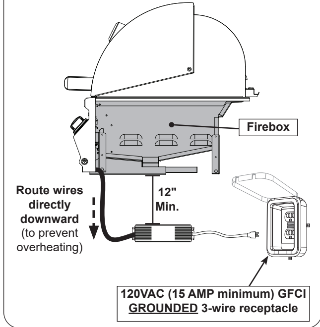
Fig. 26-1 Electrical installation
