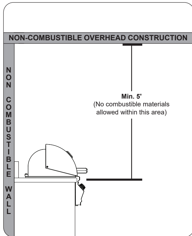
Fig. 15-1 Overhead requirements
