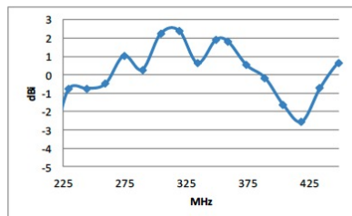
UHF gain, dBi
