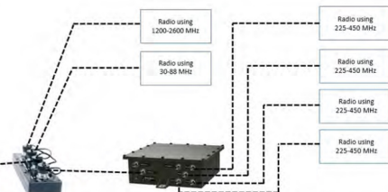
Six radio communication ports from one elevated antenna: 1 x VHF (30-88 MHz) 4 x UHF (225-450 MHz) 1 x L S Band (1200-2600 MHz) * Simultaneous transmit or receive
