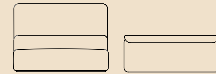
square chaise high 1820w x 700d x 1300h mm 440mm seat height
