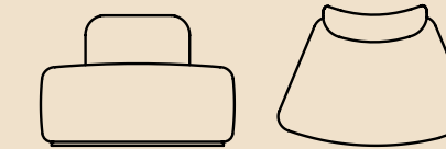
1/8 outside curve low 1030w x 700d x 700h mm 440mm seat height
