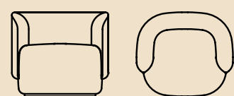
single armchair 800w x 700d x 700h mm 440mm seat height
