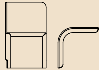
workpod screen 800w x 800d x 1300h mm
