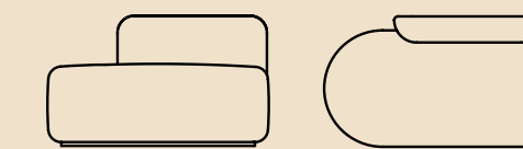
round chaise right low 1185w x 700d x 700h mm 440mm seat height
