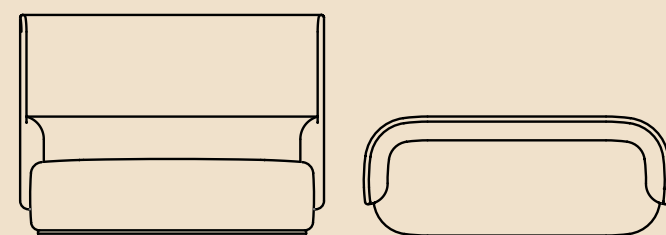
2 seat sofa high back 1800w x 700d x 1300h mm 440mm seat height
