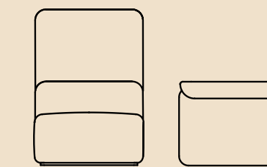
square single high 920w x 700d x 1300h mm 440mm seat height
