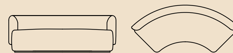
1/4 inside curve low 2040w x 900d x 700h mm 440mm seat height
