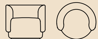
single round armchair 800w x 750d x 700h mm 440mm seat height
