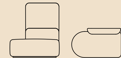
round chaise right high 1185w x 700d x 1300h mm 440mm seat height
