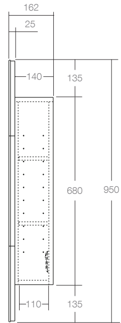
SIDE ELEVATION
