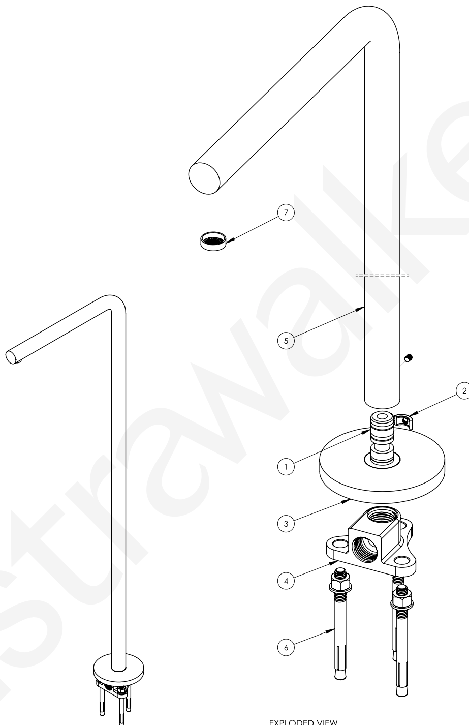
EXPLODED VIEW SCALE 1:2
