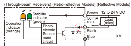
Models with NPN Output
