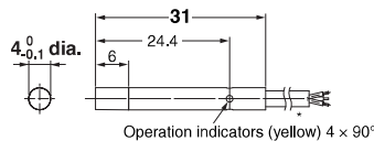
Operation indicators (yellow) 4 × 90° * 2.9-dia. vinyl-insulated round cable with 3 conductors (Conductor cross section: 0.14 mm², Insulator diameter: 0.8 mm), Standard length: 2 m Model with robot (bending-resistant) cable: 2.9-dia. vinyl-insulated round cable with 3 conductors (Conductor cross section: 0.15 mm², Insulator diameter: 1.05 mm), Standard length: 2 m
