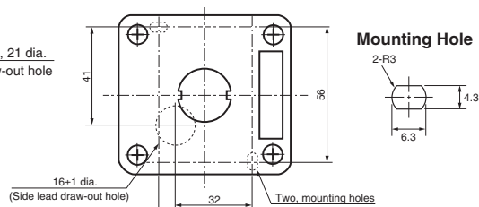
Cable Draw-out Hole (Top View)
