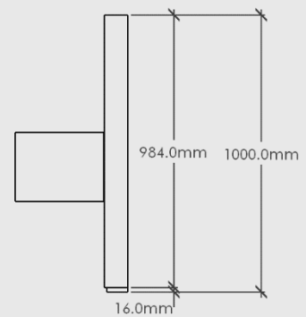
ELEVATION - SIDE
