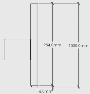
ELEVATION - SIDE
