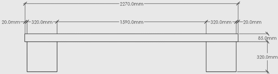
PLAN VIEW
