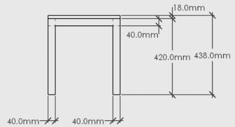
ELEVATION - SIDE
