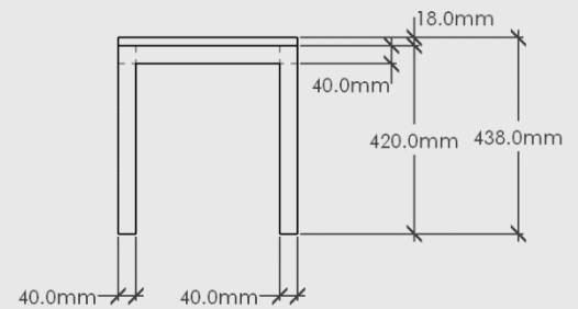
ELEVATION - SIDE
