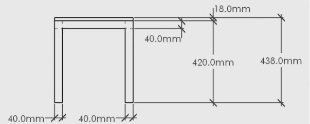
ELEVATION - SIDE
